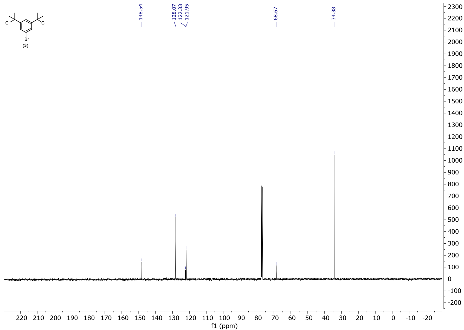
^{13}\text{C} NMR of 1-bromo-3,5-bis(1-chloro-1-methylethyl)benzene ( 3 ) (101 MHz, \text{CDCl}_3 )
